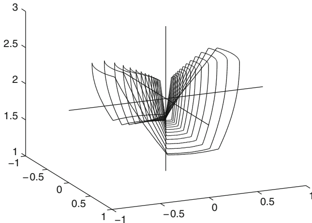
Fig. 11.1 A contour sketch of the exponent p
